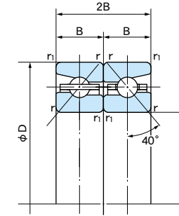
Type TBH
