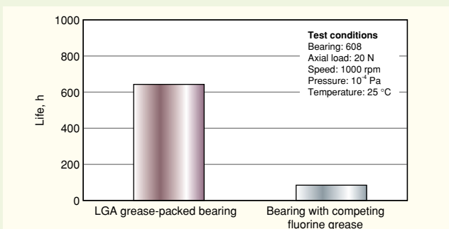
Fig. 3 Bearing durability in vacuum environment
