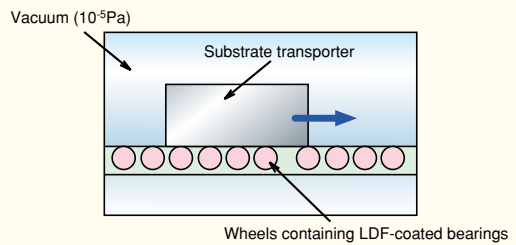
Fig. 6 Sputtering equipment
